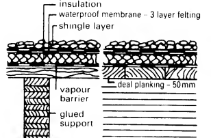
5 Warm roof with glue-laminated beams and sheathing of planed planks
